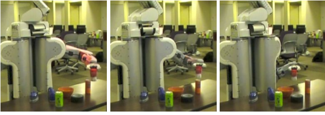
Fig. 7. A constrained motion plan being executed by the PR2 robot while picking up an object and moving it to the side. Note that the object is kept close to horizontal throughout the plan.
